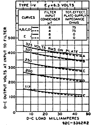
OPERATION CHARACTERISTICS
